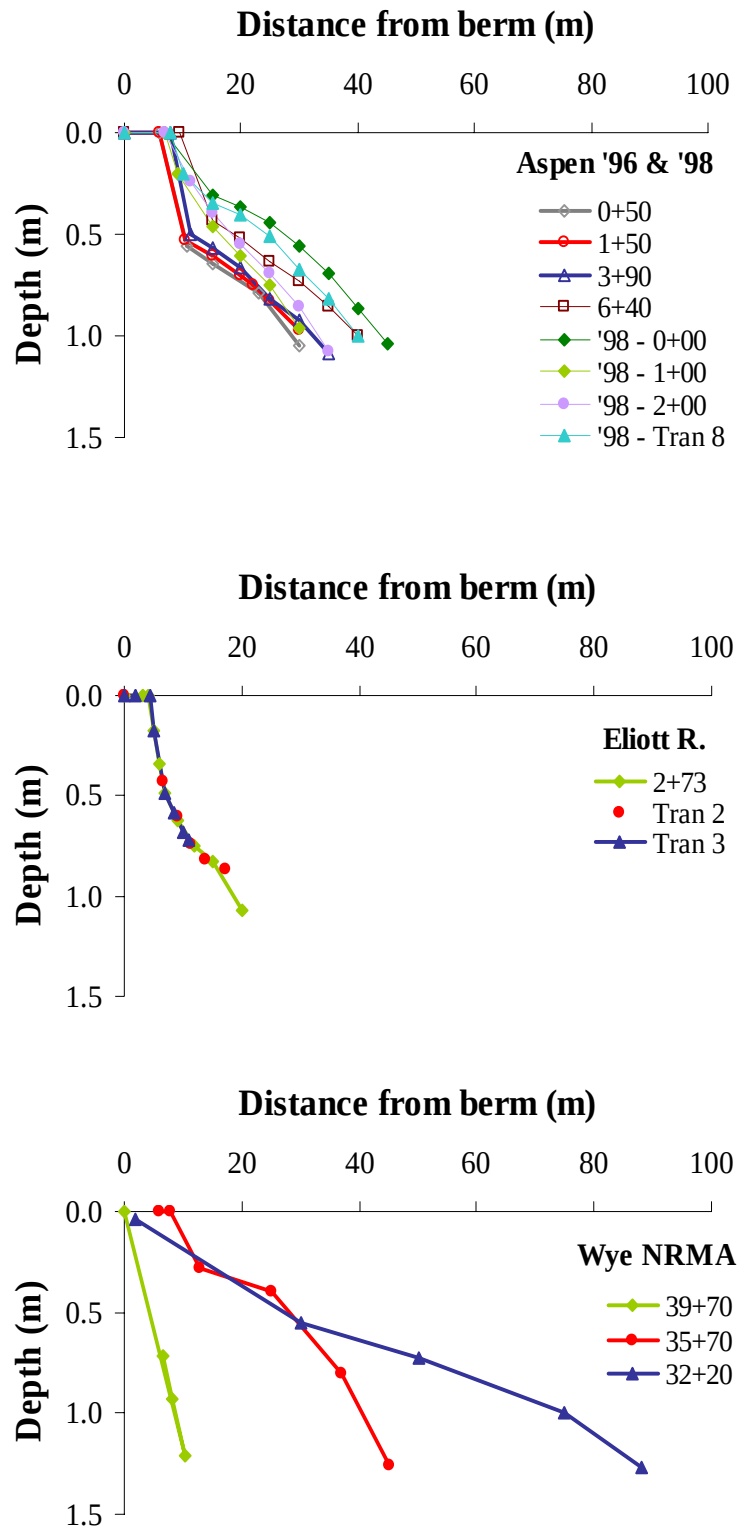
Figure 4. Present shore profiles at DNR sites. Measurements of water depth at each transect within each site. Each line represents a transect perpendicular to shore.
