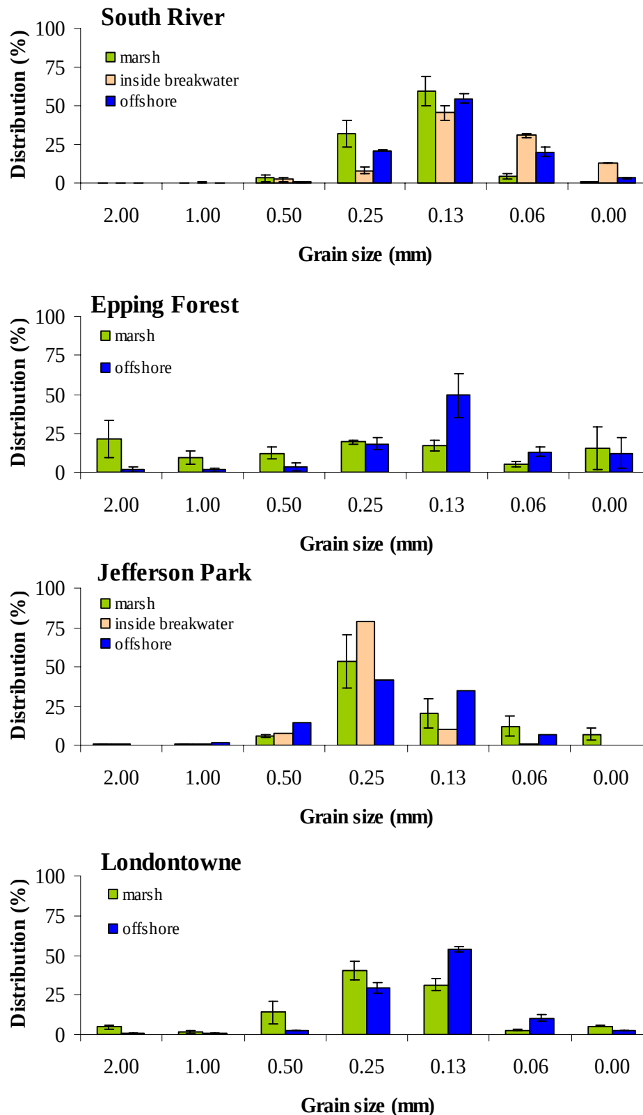
Figure 2B. Sediment Grain Size Distribution for CBT sites. Offshore samples were collected at a depth of approximately 0.7 m. Grain size classes are as follows: gravel (2.00 mm), very coarse sand (1.00 mm), coarse sand (0.5 mm), medium sand (0.25 mm), fine sand (0.13 mm), very fine sand (0.063 mm) and silt + clay (0.00 mm).
