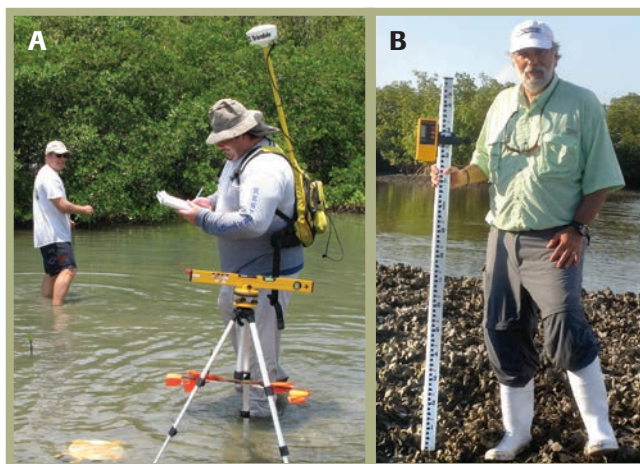
Figure 12. (A & B) Using a tripod-mounted laser level to measure reef height.
